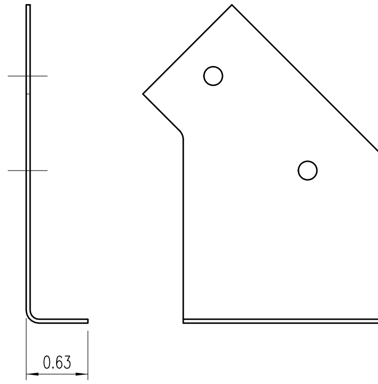
-15 PROFILE DETAIL
