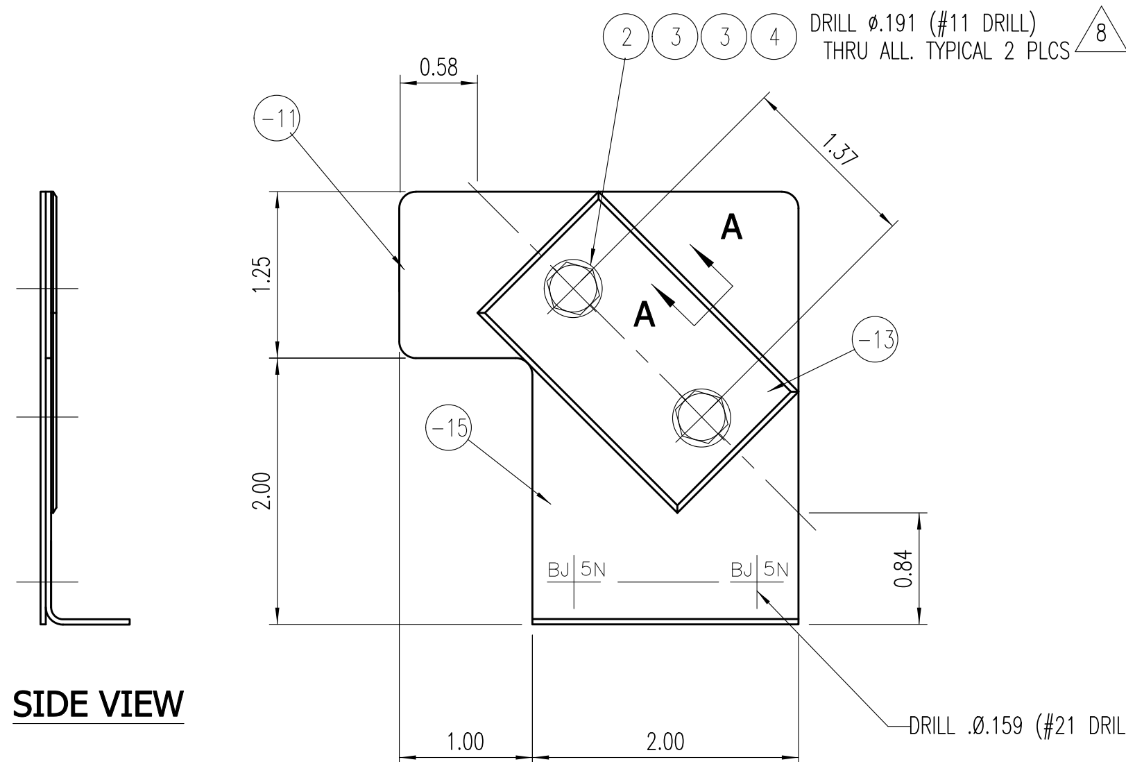
-1 ASSEMBLY PLAN VIEW
